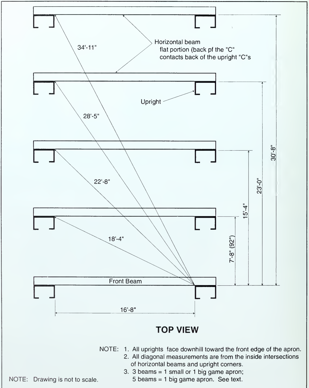
Figure 3. Critical measurements for guzzler aprons.
